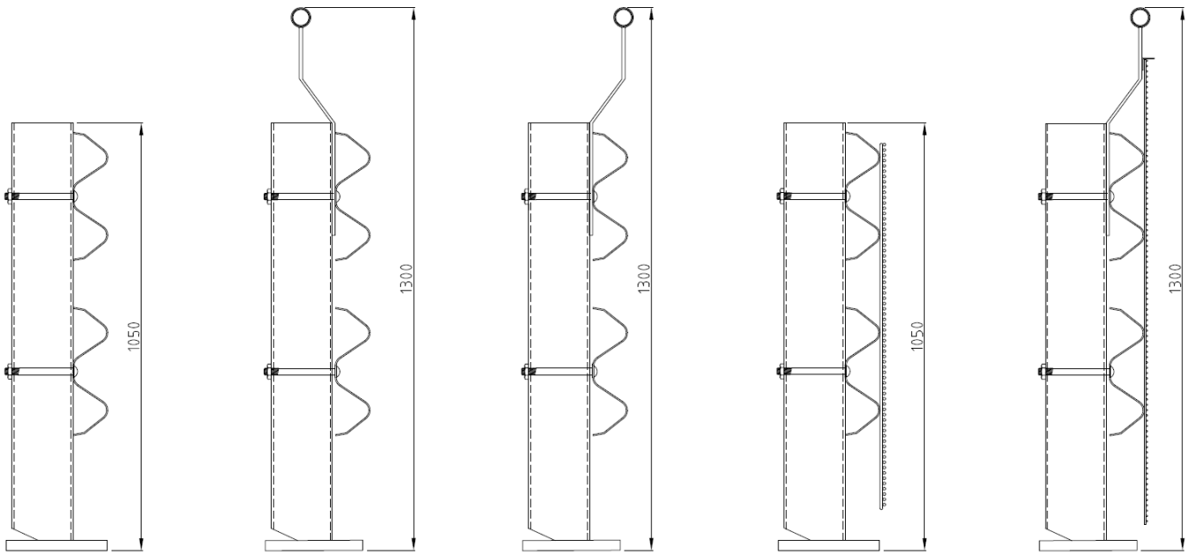
Rhino-Stop Truck Guard Type 2 Guardrail & Offside Balustrade
