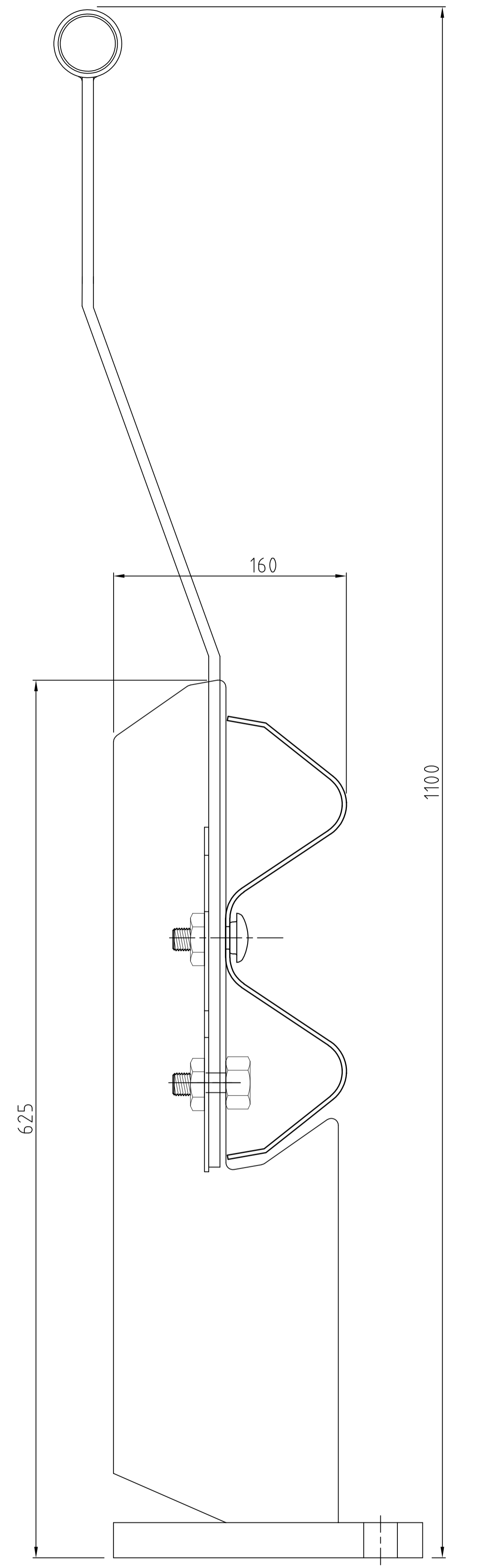
POST ELEVATION
