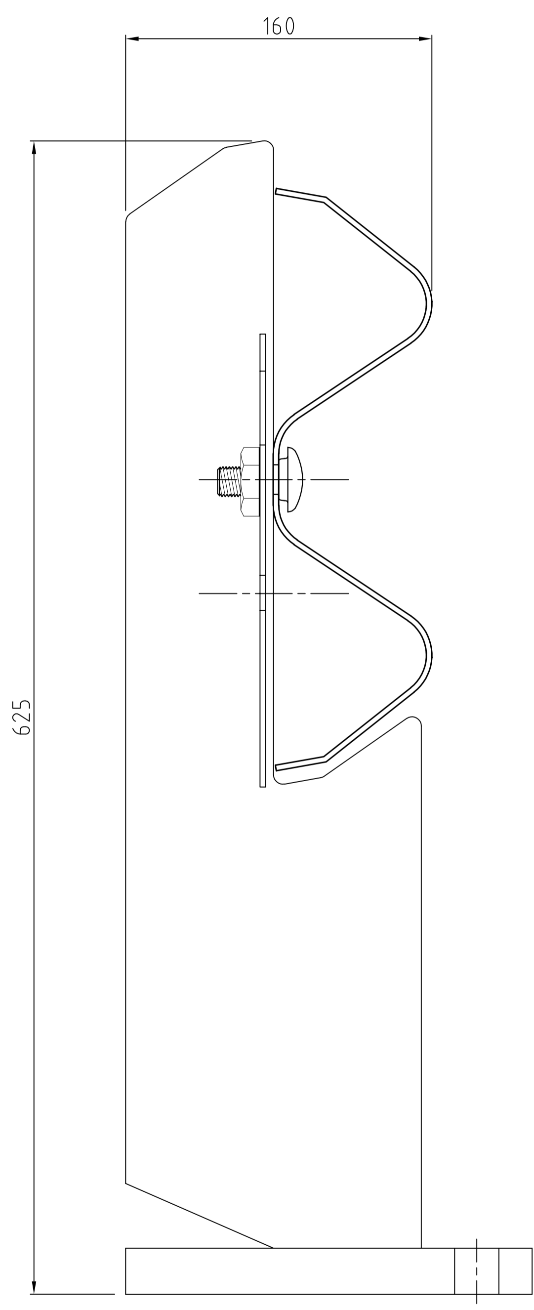
POST ELEVATION
