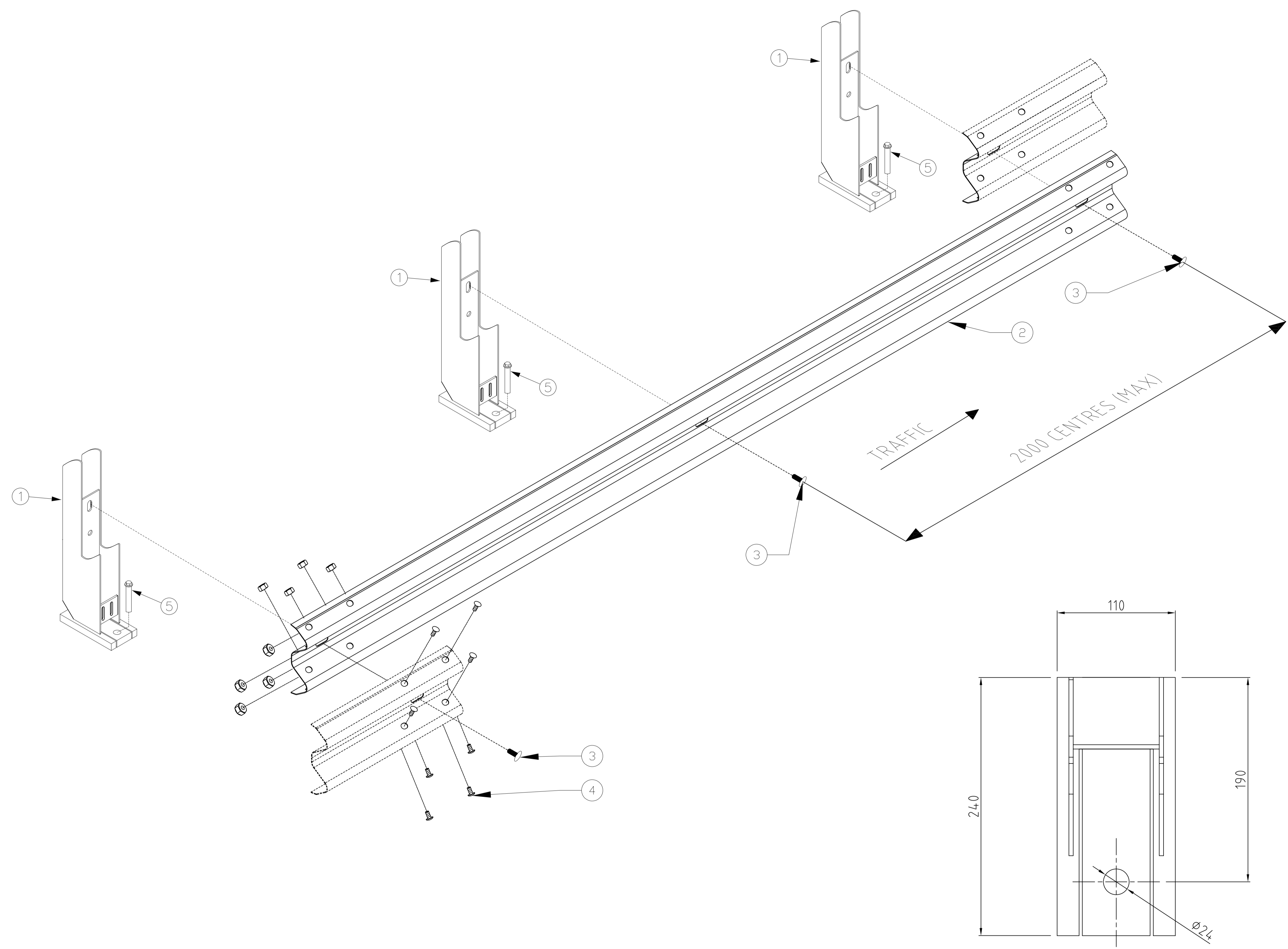
BASE PLATE DETAIL
